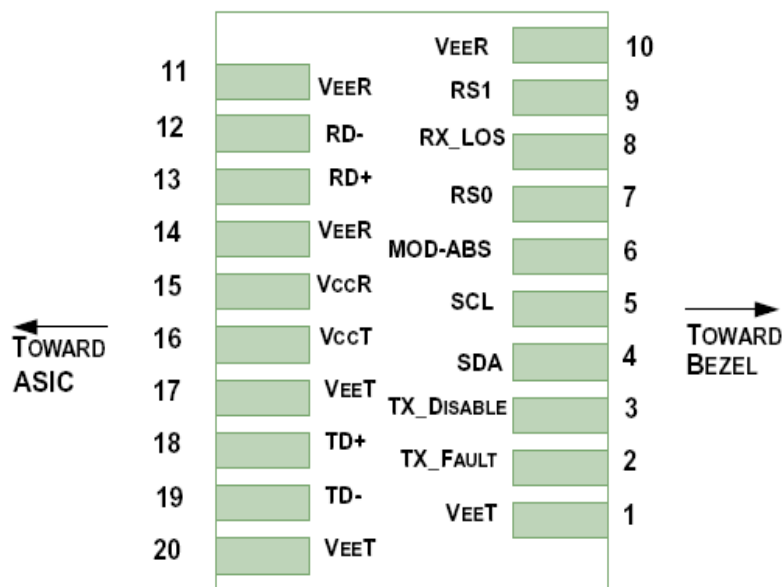
Figure 3, Pin View
